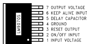
7-Lead TO-263 Surface Mount Package
